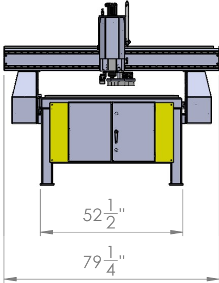
STANDARD MACHINE
